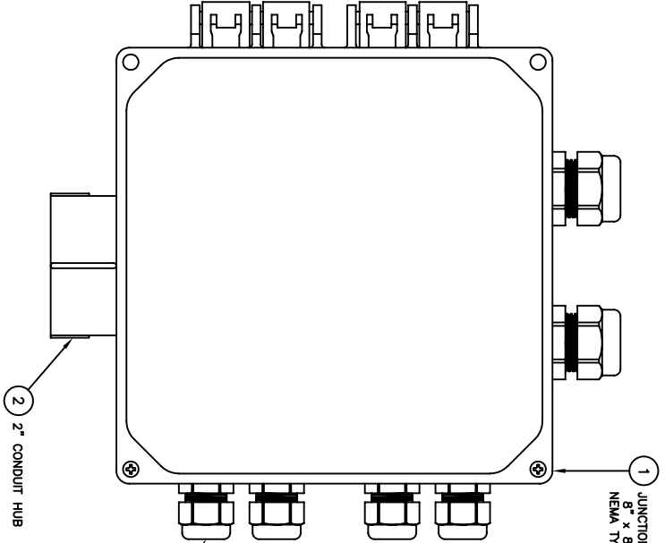
3 CORD GRIP: \frac{1}{2} " NPT THD. CABLE RANGE: 0.170"-0.470" (4 REQ'D)
