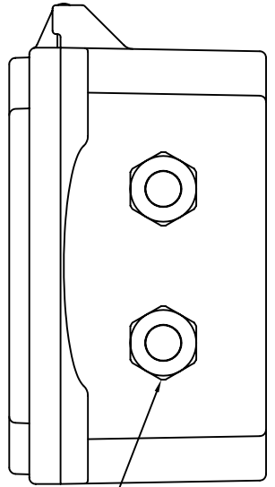
4 CORD GRIP: \frac{3}{4} " NPT THD. CABLE RANGE: 0.450"-0.709" (2 REQ'D)
