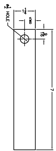
① MOUNTING BRACKET 11 GA., 304 SST PLATE
