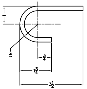
③ HOOK 304 SST ROD 5/16"
